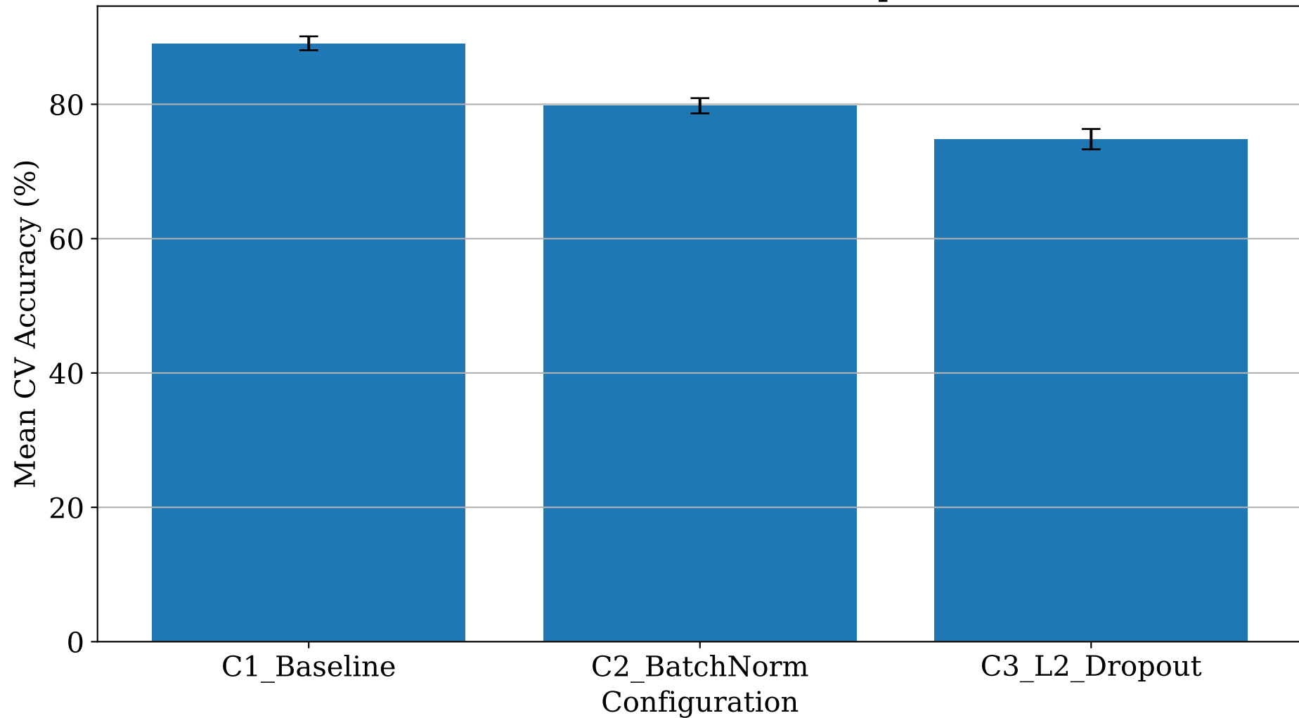
5-Fold Cross-Validation Comparison
